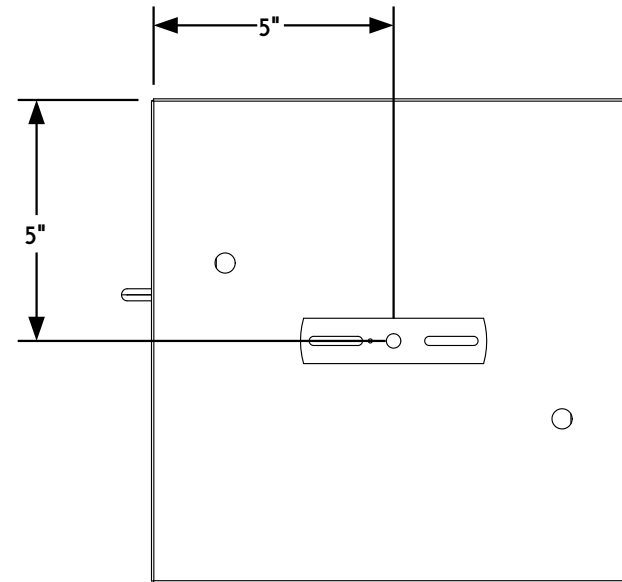
② CEILING LIGHT MOUNT SURFACE VIEW
