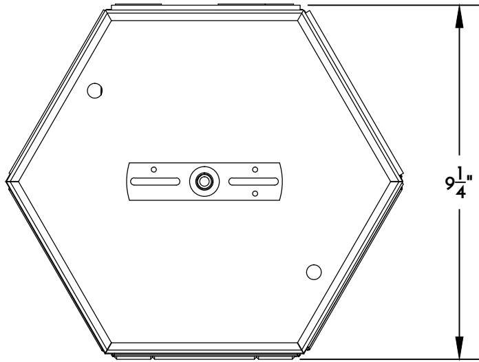
1 CEILING LIGHT PLAN VIEW
