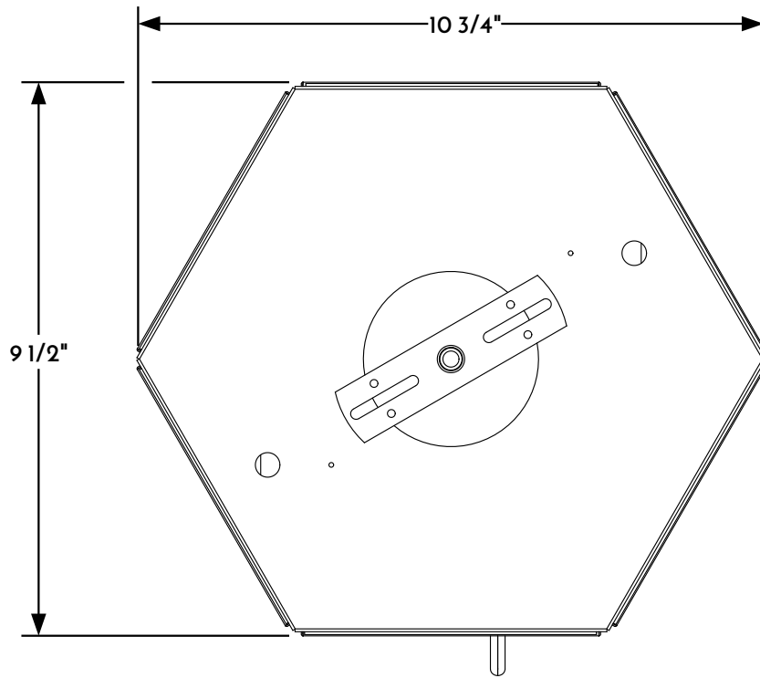
④ CEILING LIGHT PLAN VIEW
