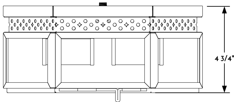
① CEILING LIGHT ELEVATION VIEW
