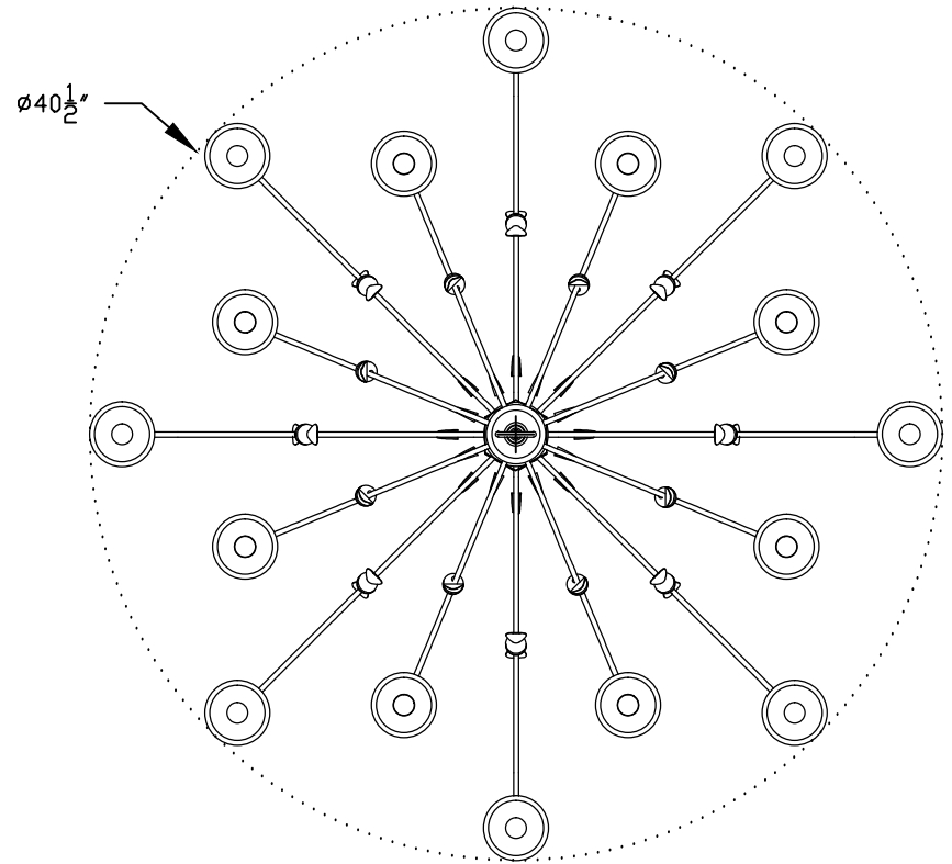
2 HANGING CHANDELIER PLAN VIEW
