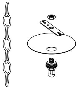
3 HANGING CHANDELIER CANOPY ASSEMBLY
