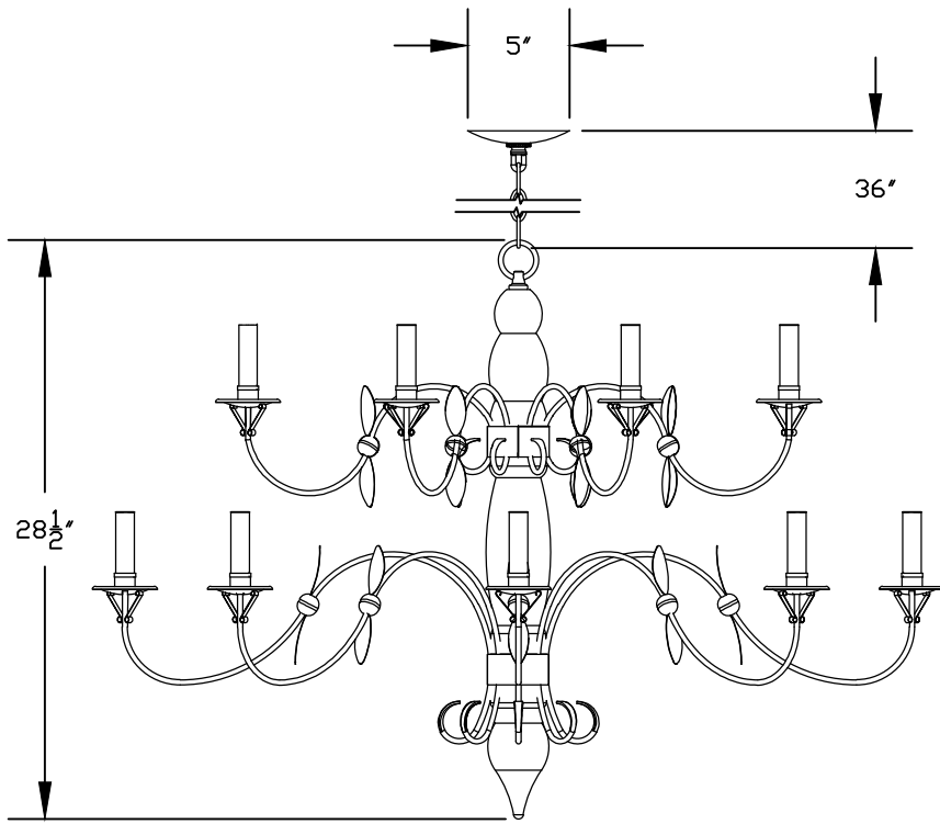
1 HANGING CHANDELIER ELEVATION VIEW
