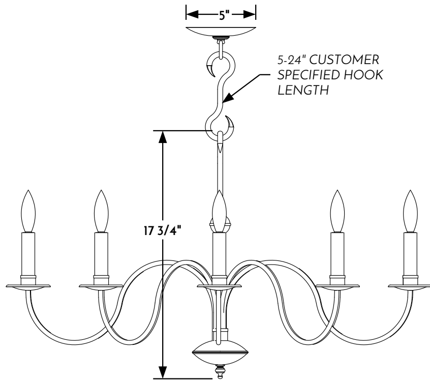
① HANGING CHANDELIER ELEVATION VIEW
