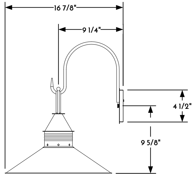
② WALL PENDANT RIGHT ELEVATION VIEW
