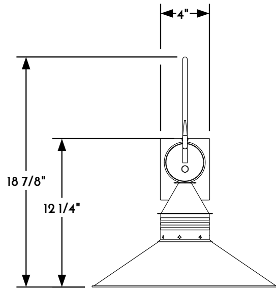
① WALL PENDANT FRONT ELEVATION VIEW
