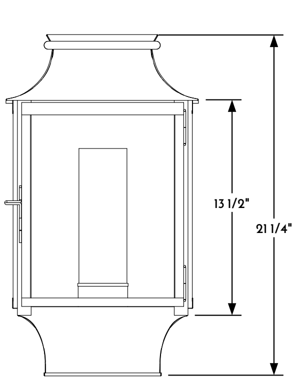
① WALL LANTERN FRONT ELEVATION VIEW
