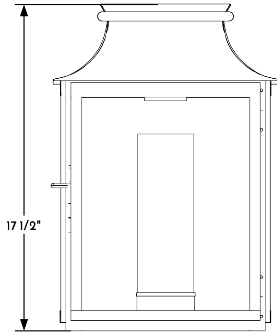
① WALL LANTERN FRONT ELEVATION VIEW
