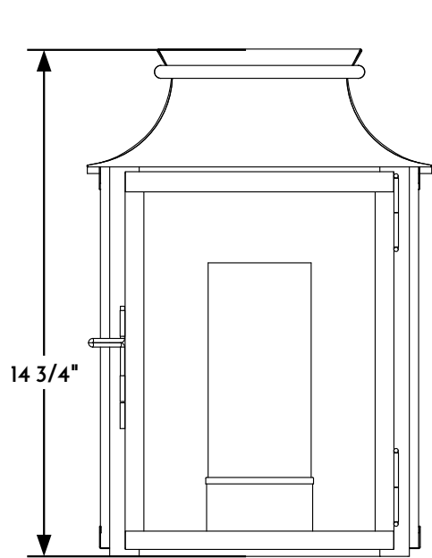
① WALL LANTERN FRONT ELEVATION VIEW
