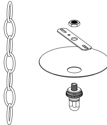
④ HANGING LANTERN CANOPY ASSEMBLY
