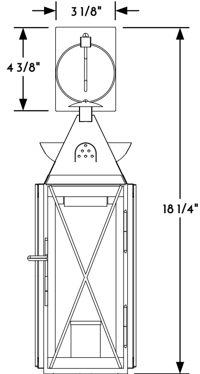
① WALL LANTERN FRONT ELEVATION VIEW
