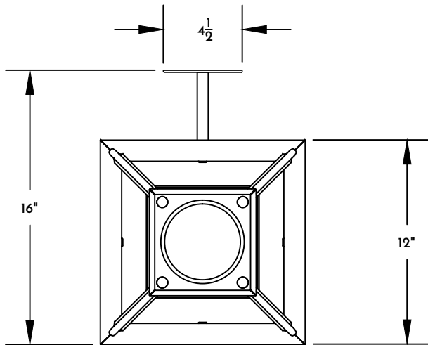
③ WALL LANTERN PLAN VIEW
