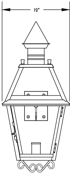
① WALL LANTERN FRONT ELEVATION VIEW
