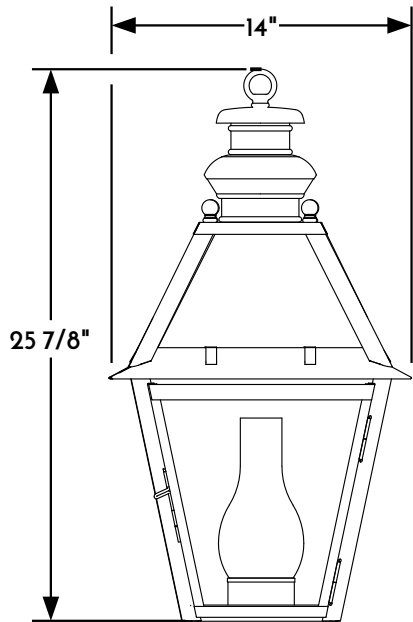
① HANGING LANTERN FRONT ELEVATION VIEW
