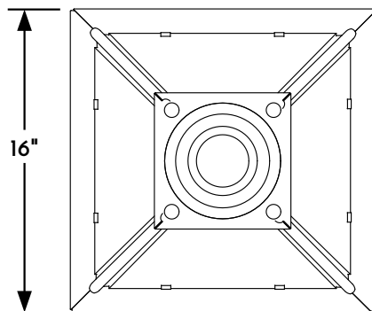
③ POST LANTERN PLAN VIEW
