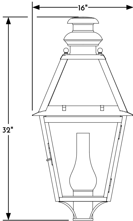
① POST LANTERN FRONT ELEVATION VIEW
