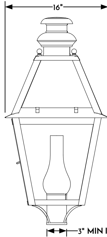
② POST LANTERN RIGHT ELEVATION VIEW
