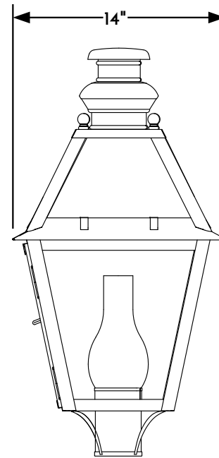
② POST LANTERN RIGHT ELEVATION VIEW
