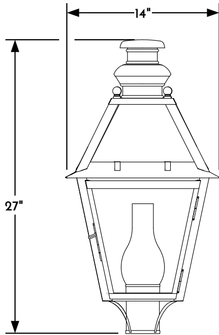
① POST LANTERN FRONT ELEVATION VIEW
