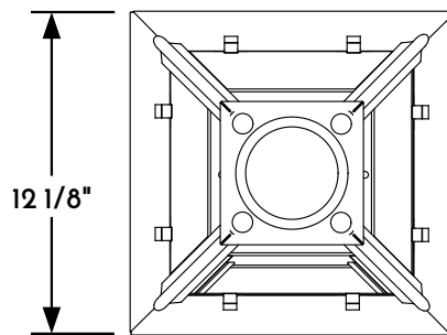
③ POST LANTERN PLAN VIEW
