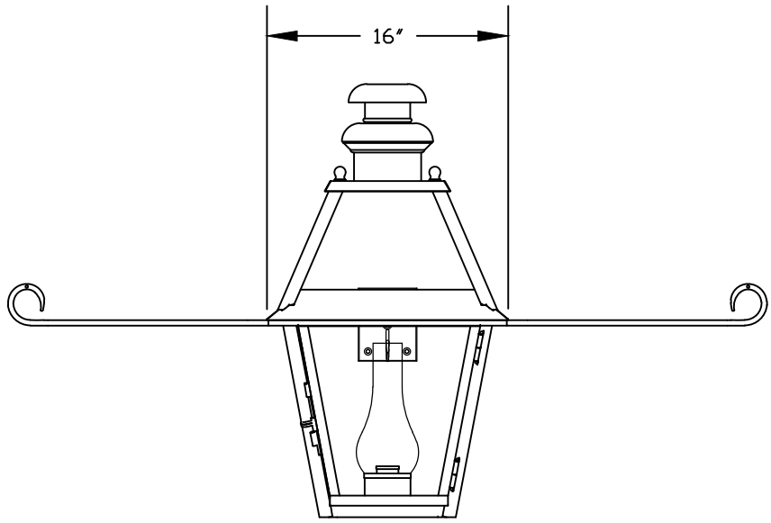
① WALL LANTERN FRONT ELEVATION VIEW
