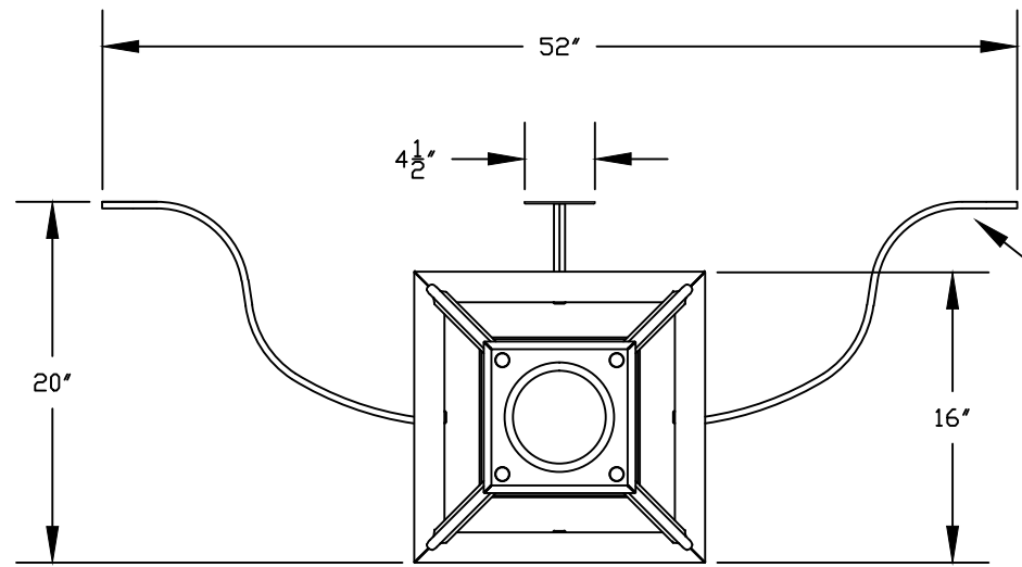
③ WALL LANTERN PLAN VIEW
