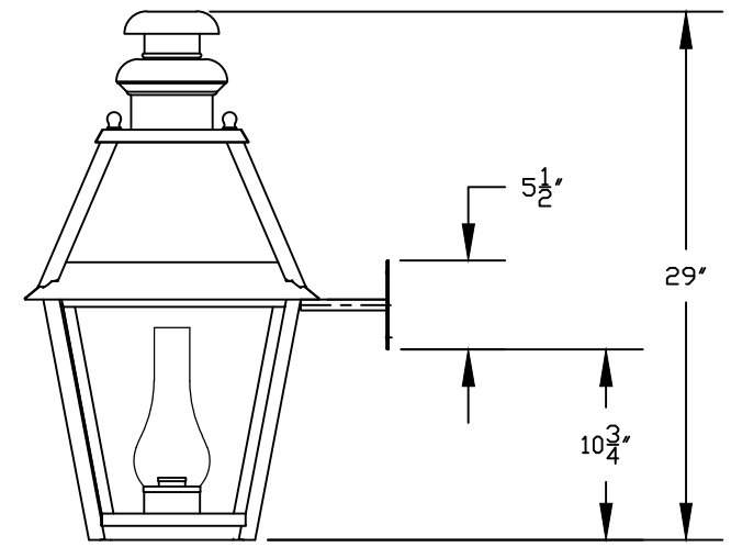
② WALL LANTERN RIGHT ELEVATION VIEW
