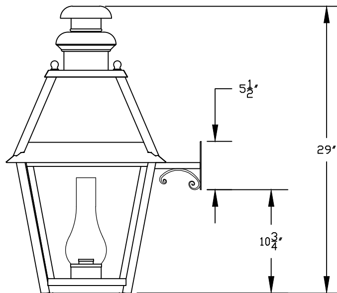
② WALL LANTERN RIGHT ELEVATION VIEW
