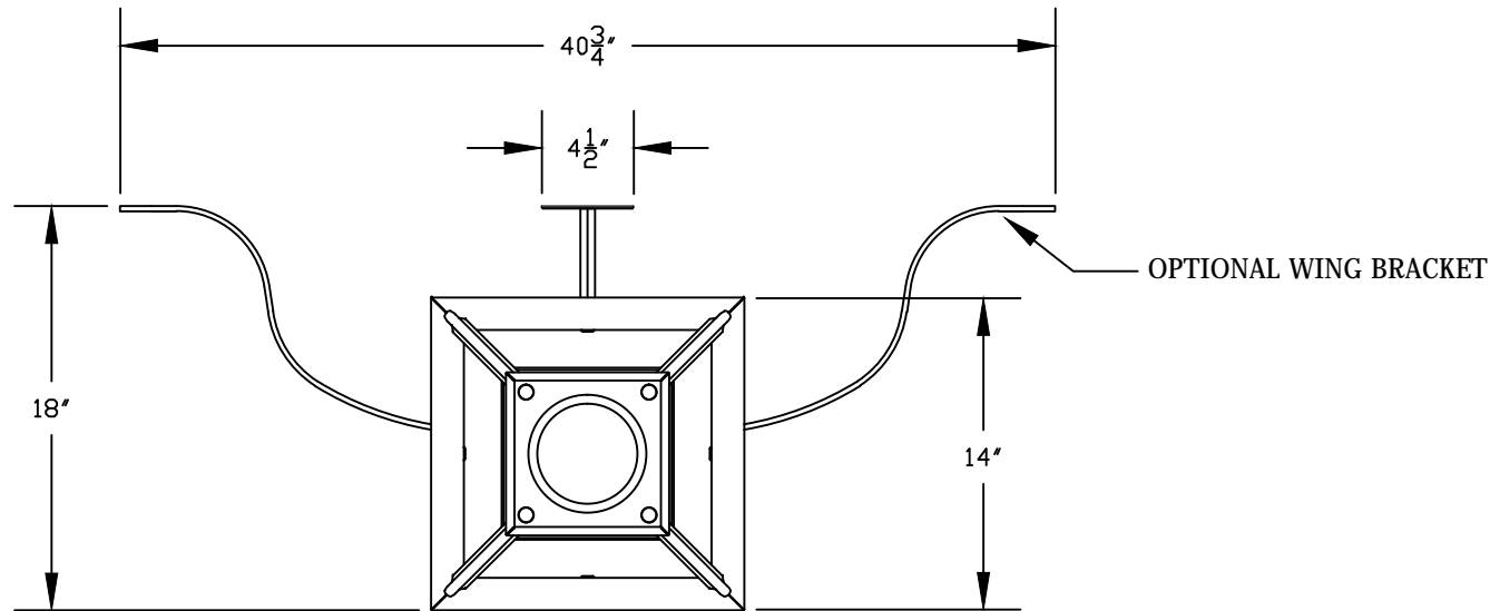
3 WALL LANTERN PLAN VIEW
