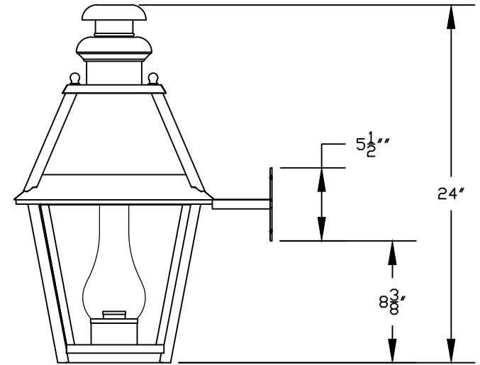
2 WALL LANTERN RIGHT ELEVATION VIEW
