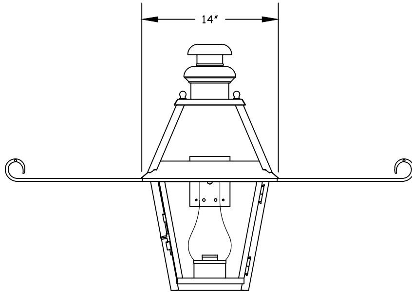
1 WALL LANTERN FRONT ELEVATION VIEW
