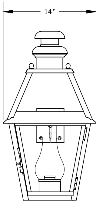
1 WALL LANTERN FRONT ELEVATION VIEW
