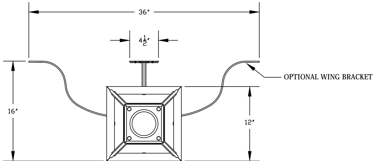
③ WALL LANTERN PLAN VIEW
