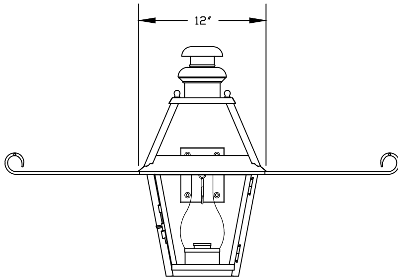
① WALL LANTERN FRONT ELEVATION VIEW
