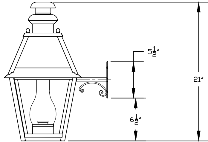
② WALL LANTERN RIGHT ELEVATION VIEW
