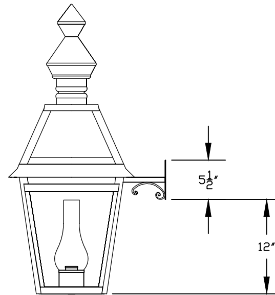
② WALL LANTERN RIGHT ELEVATION VIEW
