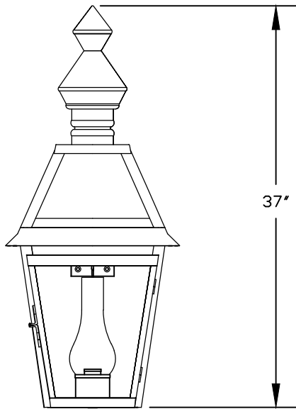
① WALL LANTERN FRONT ELEVATION VIEW
