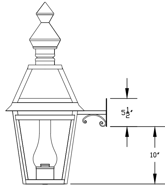
② WALL LANTERN RIGHT ELEVATION VIEW
