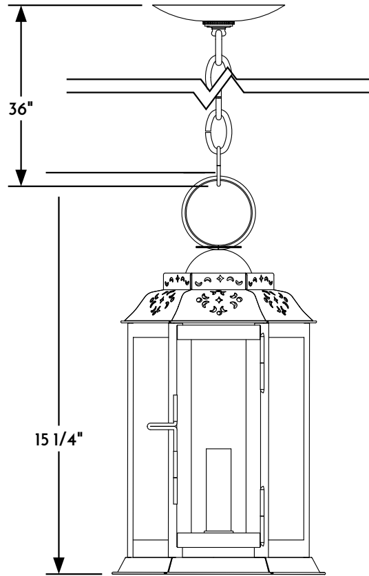
① HANGING LANTERN FRONT ELEVATION VIEW
