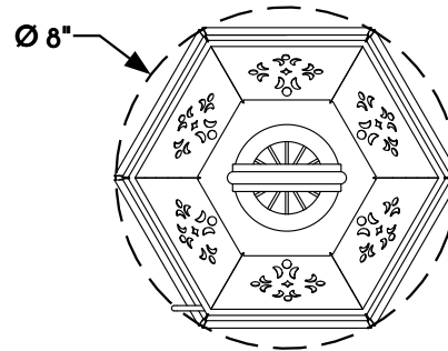
③ HANGING LANTERN PLAN VIEW
