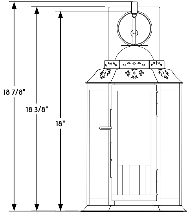
① WALL LANTERN FRONT ELEVATION VIEW
