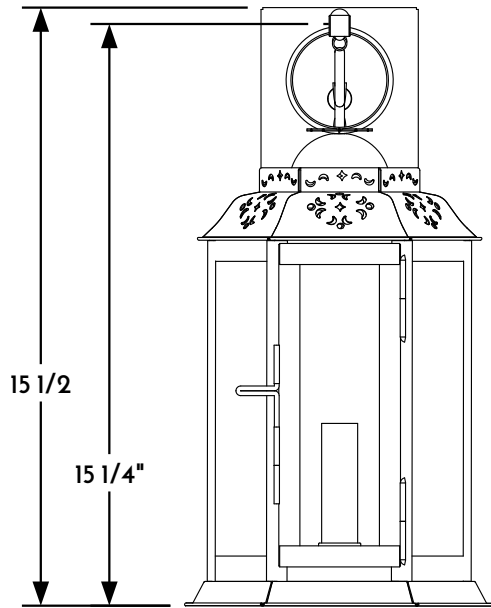
① WALL LANTERN FRONT ELEVATION VIEW
