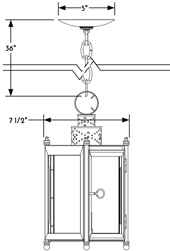
① HANGING LANTERN FRONT ELEVATION VIEW
