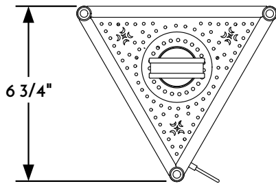
④ HANGING LANTERN PLAN VIEW
