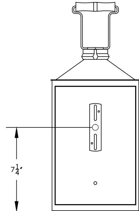
② WALL LANTERN REAR ELEVATION VIEW
