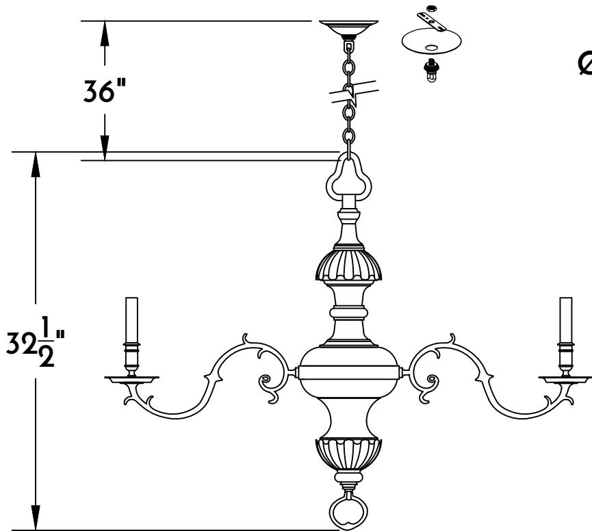
① CHANDELIER SIDE ELE.
