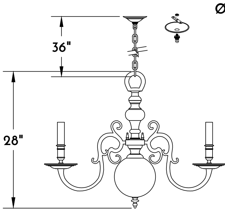
① CHANDELIER FRONT ELE.
