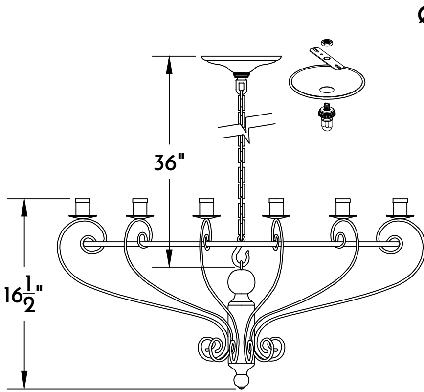
① CHANDELIER SIDE ELE.
