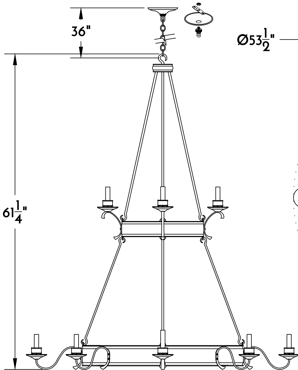
① CHANDELIER SIDE ELE.
