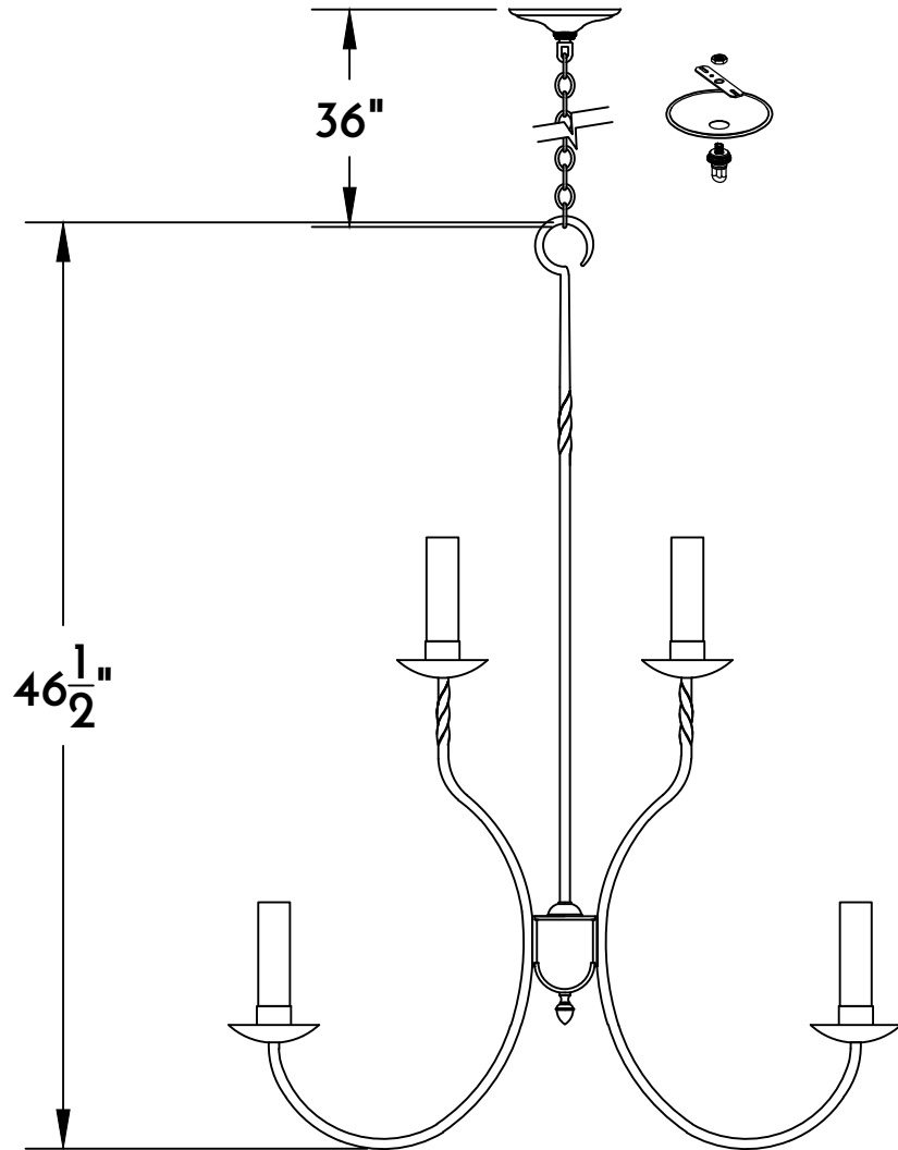
① CHANDELIER LANTERN SIDE ELE.
