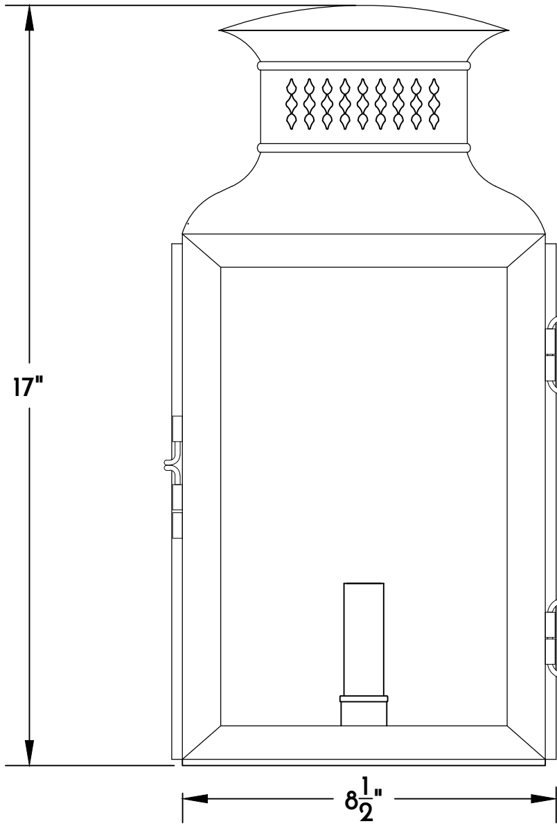
① WALL LANTERN FRONT VIEW
