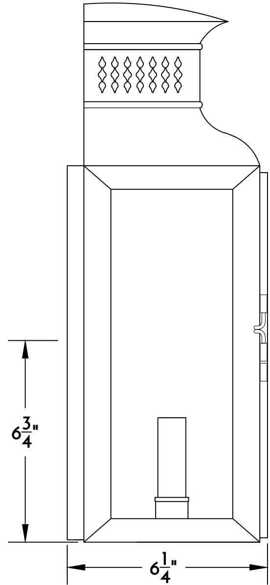
② WALL LANTERN SIDE VIEW
