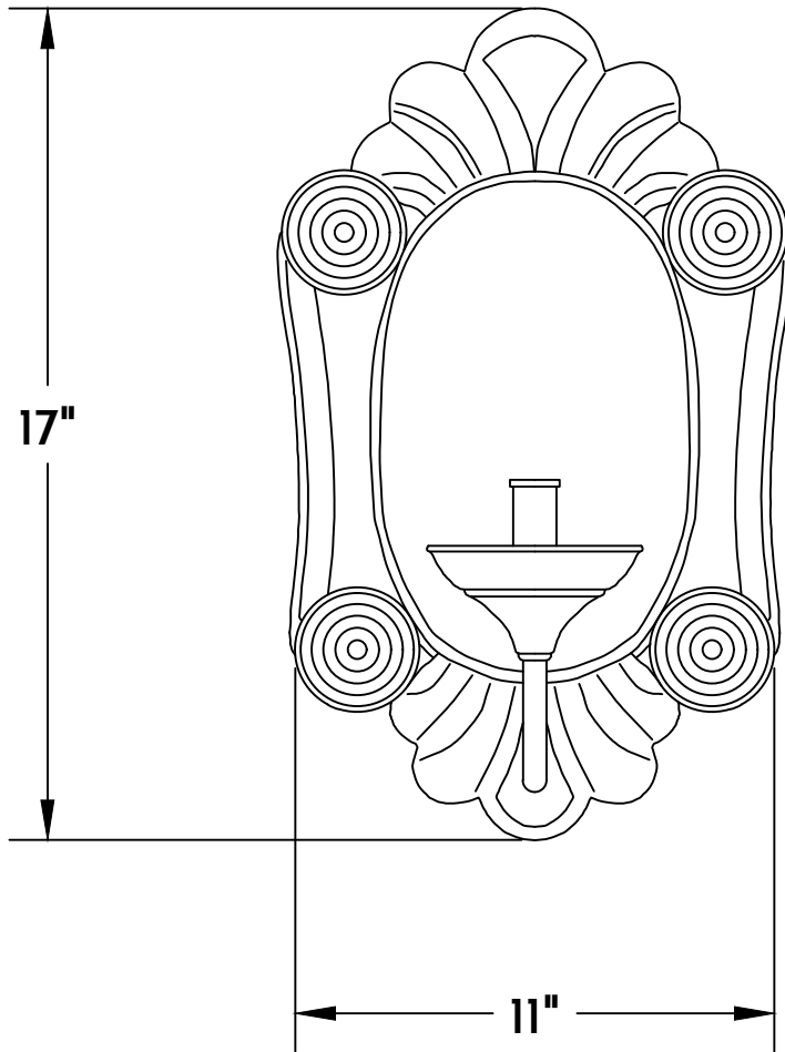
① SCONCE FRONT VIEW
