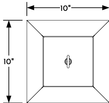
② HANGING LANTERN PLAN VIEW
