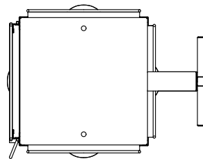
⑤ WALL LANTERN BOTTOM VIEW
