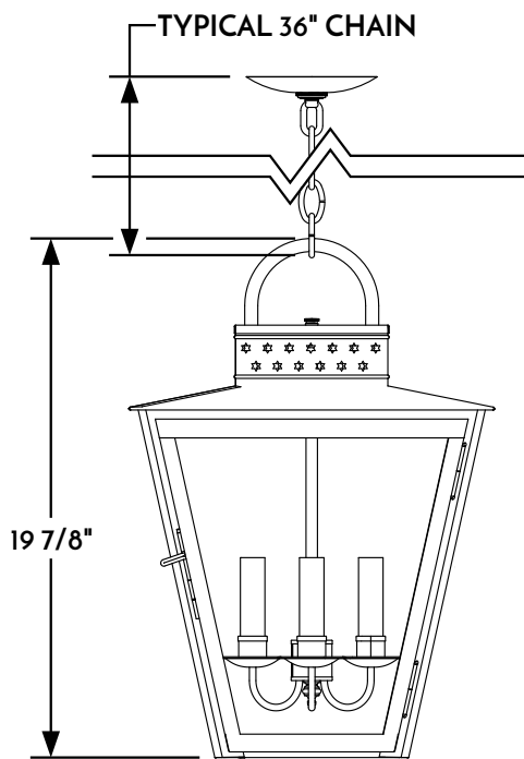
① HANGING LANTERN FRONT ELEVATION VIEW
