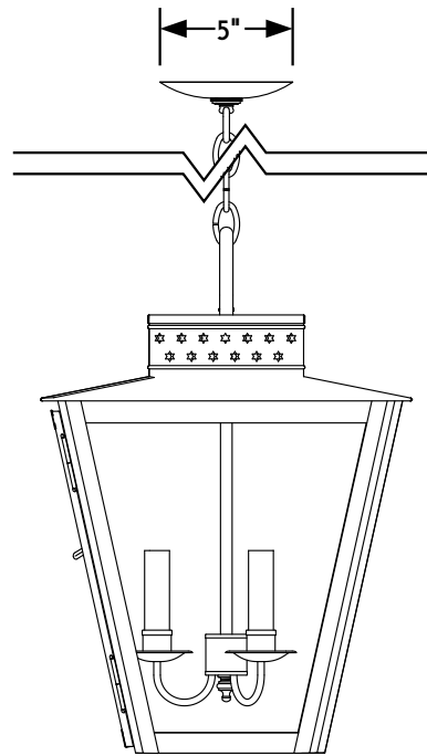
② HANGING LANTERN RIGHT ELEVATION VIEW
