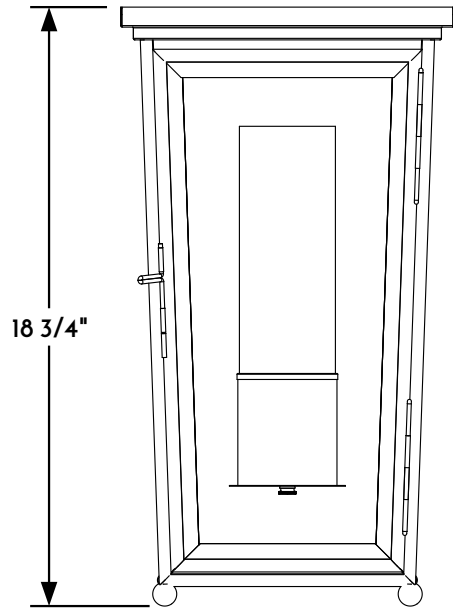
① WALL LANTERN FRONT ELEVATION VIEW
