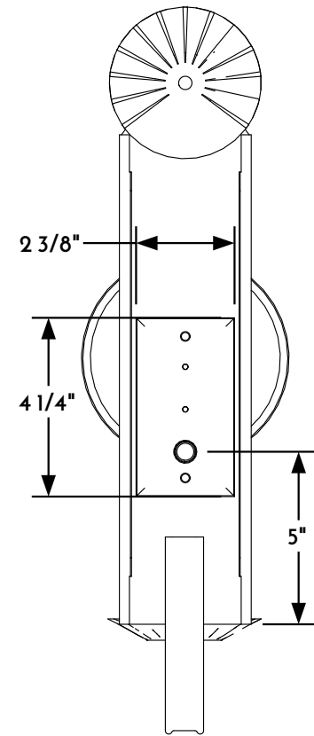
③ WALL SCONCE REAR ELEVATION VIEW
