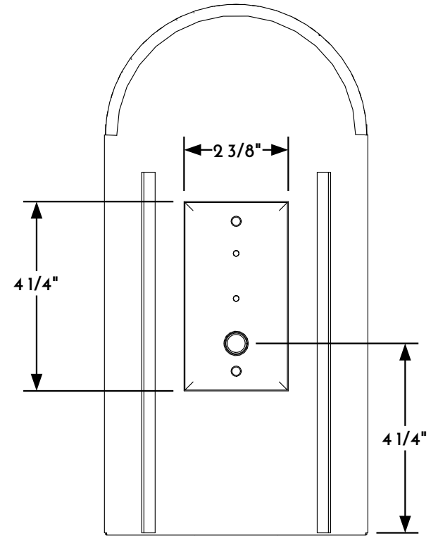
③ WALL SCONCE REAR ELEVATION VIEW
