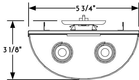
④ WALL SCONCE PLAN VIEW
