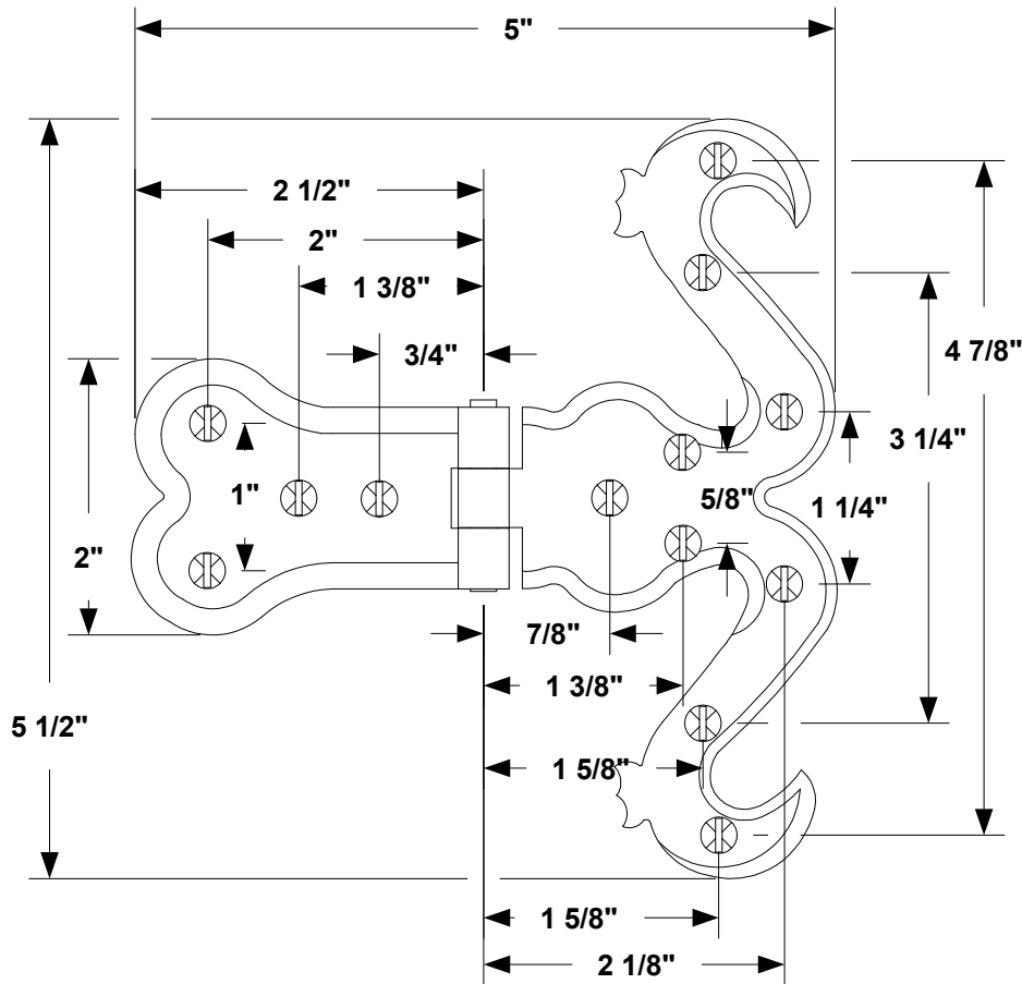
1 FRONT VIEW
