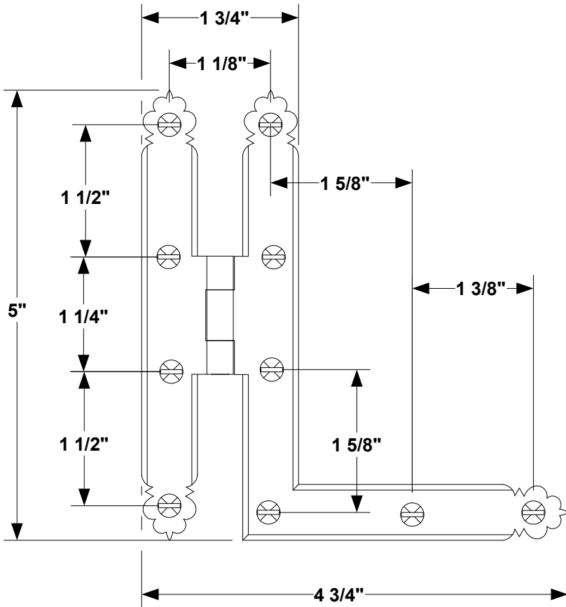
1 FRONT VIEW
