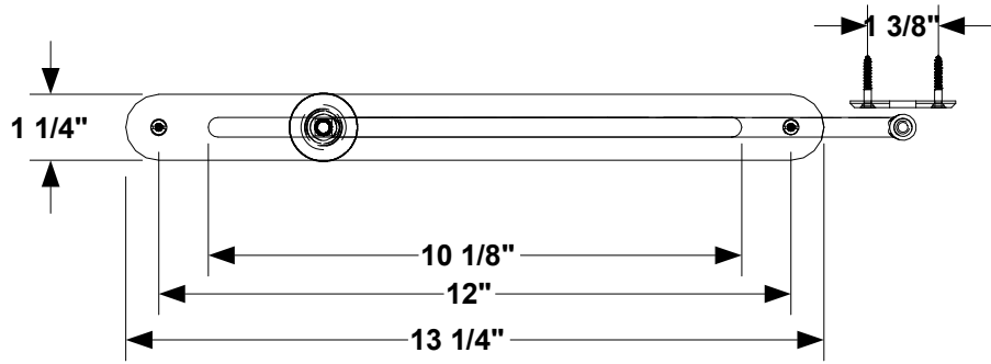
2 TOP VIEW
