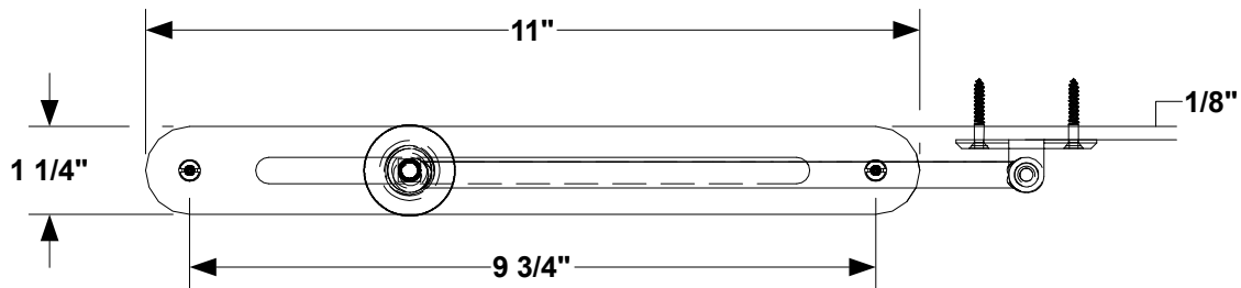
2 SIDE VIEW
