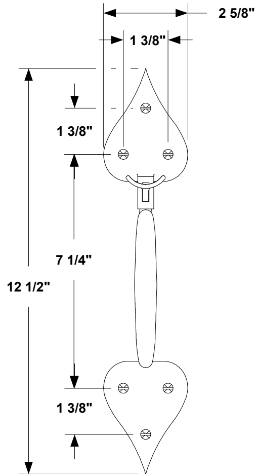
1 FRONT VIEW
