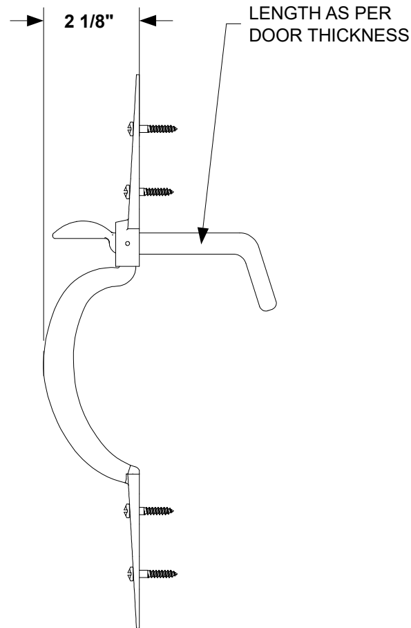
2 SIDE VIEW
