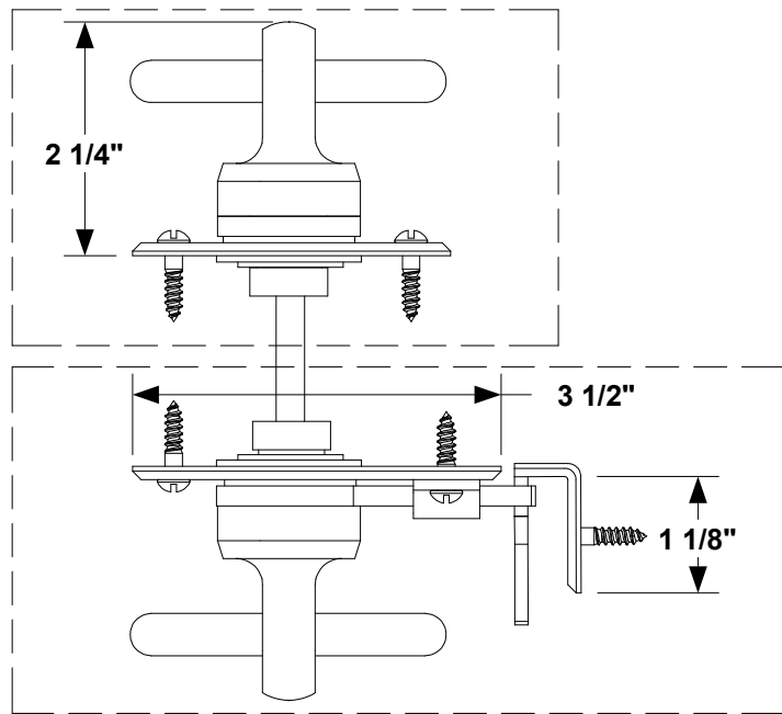
3 TOP VIEW
