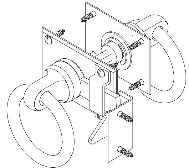
3 ISOMETRIC VIEW
