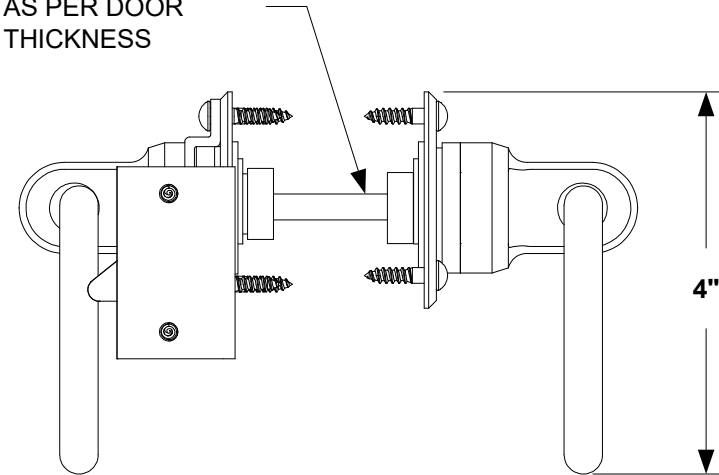
2 SIDE VIEW
