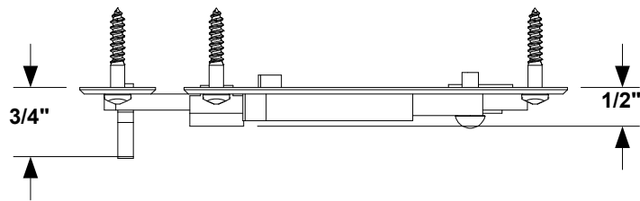
1 TOP VIEW
