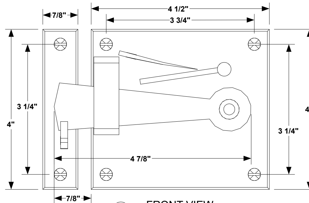
2 FRONT VIEW
