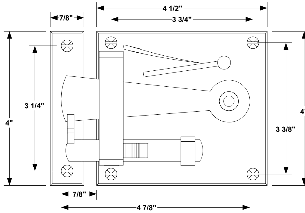
2 FRONT VIEW
