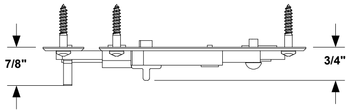
1 TOP VIEW
