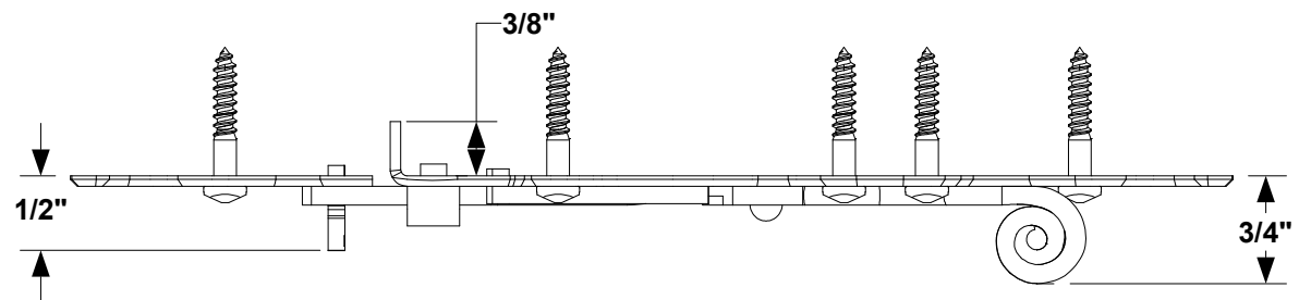
1 TOP VIEW
