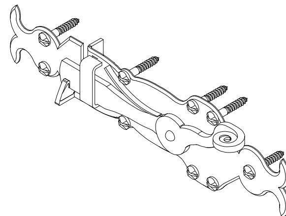
3 ISOMETRIC VIEW
